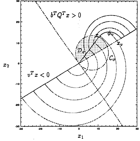
Figure 2: Trajectories under the proposed VS control for the torque generation continuous model.
