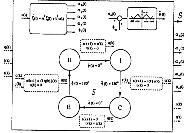
Figure 1: Hybrid model for a single cylinder.
