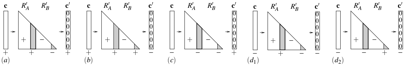
Figure 2. The four possible signature changes of \mathbf{c} , \mathbf{c}' , and the resulting possible signatures J' (after zero-c , before sorting). Only columns m-d and d of R may have changed signature.
