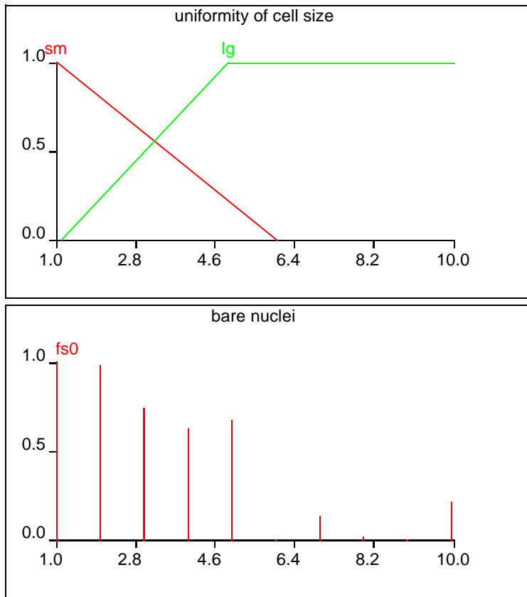
Figure 3: Membership functions for the metric variable x_2 and the categorical variable x_6 after training
