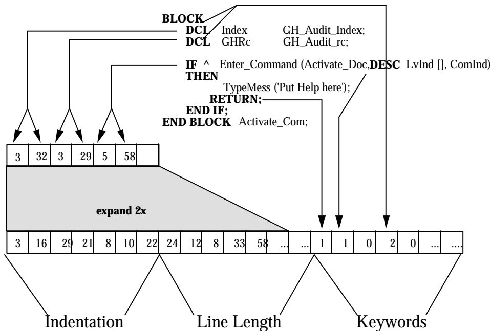
Figure 1: The representation of a block of code, as used in the clone detector
