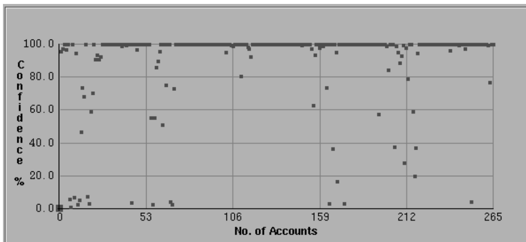
Figure 3: A visual representation of unseen fraudulent profiles. The confidence value measures the degree to which the network identifies the profile as fraudulent.
