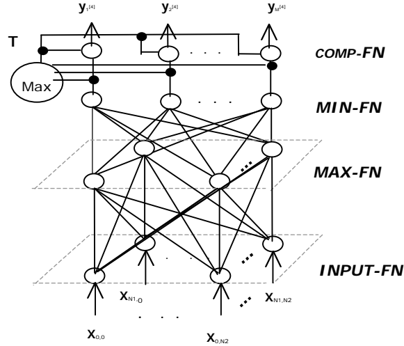
Figure 2: Four-layer feedforward fuzzy neural network
