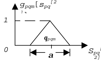
Figure 3: The output function of a MAX-FN in the second layer.
