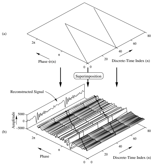
Figure 9: a) Cubic phase contour (wrapped); b) TSWI synthesis: re-sampling of the interpolated 2-D CW surface with the proposed phase track to create the 1-D reconstructed residue.
