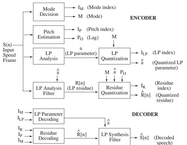
Figure 1: A linear prediction based multimode VBR codec.
