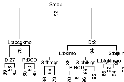
Figure 3. Global HSR decision tree
