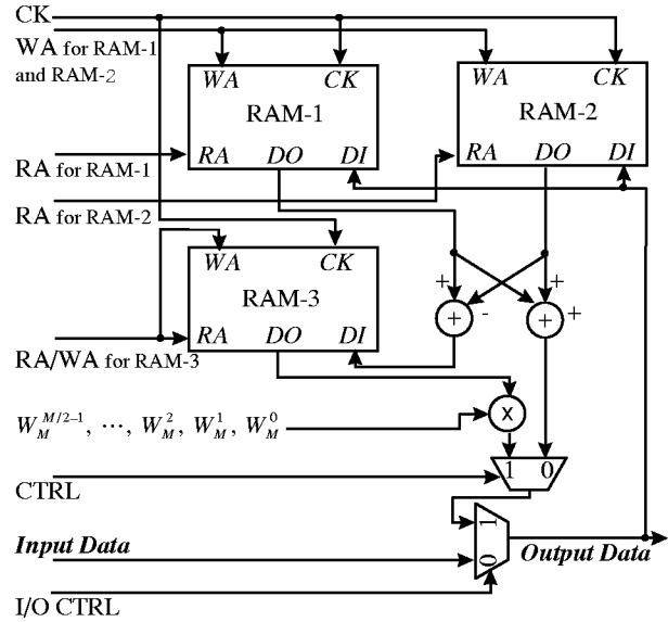
Fig. 1. A memory-based architecture for FFT computation.
