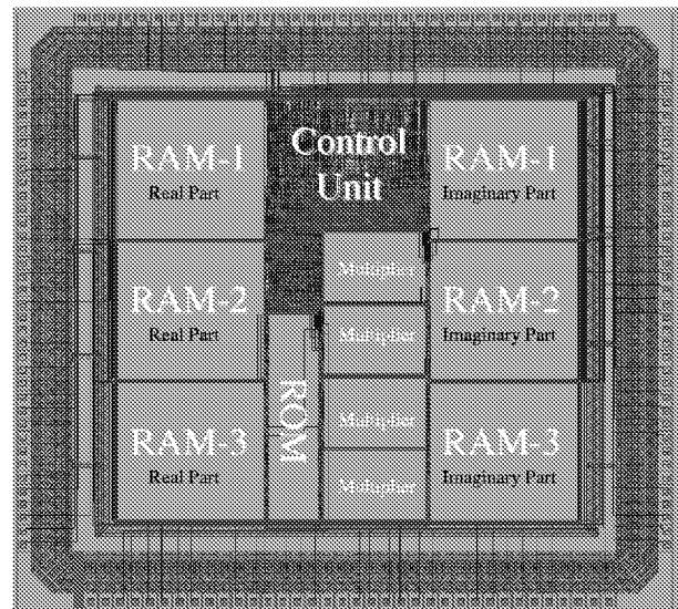
Fig. 2. A chip layout of the proposed 512-point FFT architecture.
