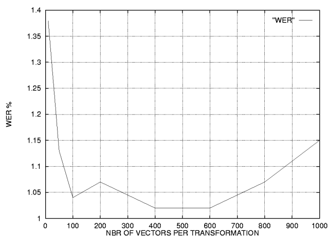
Figure 1: WER as function of minimum number of vectors per transformation
