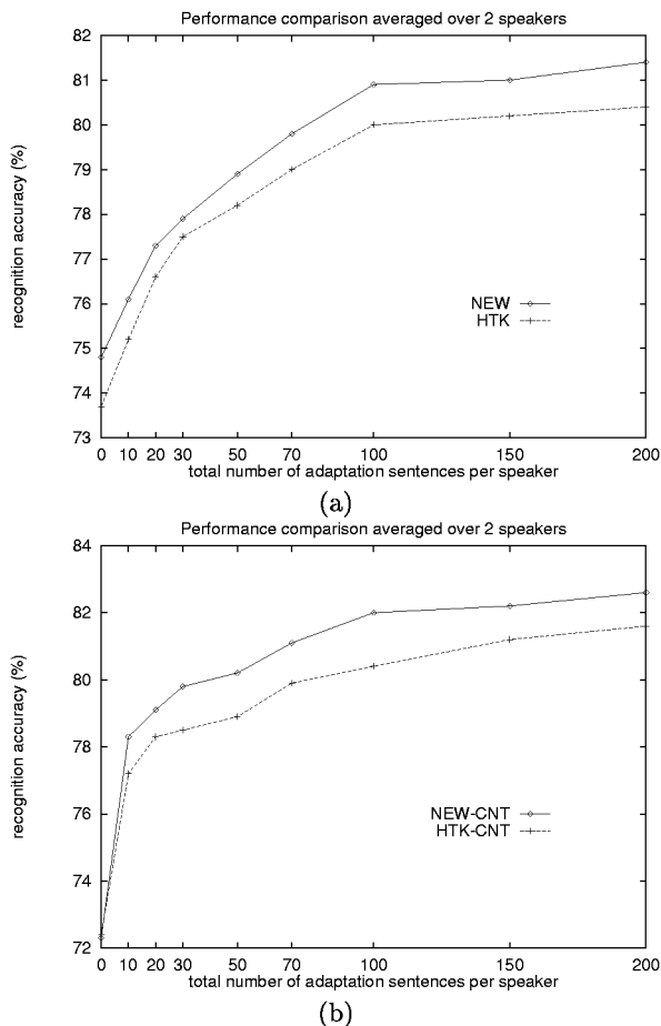
Figure 1: Performance (syllable accuracy in %) comparison averaged over 2 testing speakers as a function of number of available adaptation sentences per speaker: (a) HTK vs. New decision-tree construction with normalization, (b) HTK plus condition-normalized training (CNT) vs. New decision-tree plus CNT.
