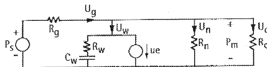
Figure 1: Low-frequency equivalent circuit used by HLSyn to calculate the intraoral pressure P_m in the vocal tract, and the flows through the glottis, nasal cavity, and supraglottal constriction ( U_g , U_n , and U_c respectively), and the flow U_w due to displacement of the vocal-tract walls.
