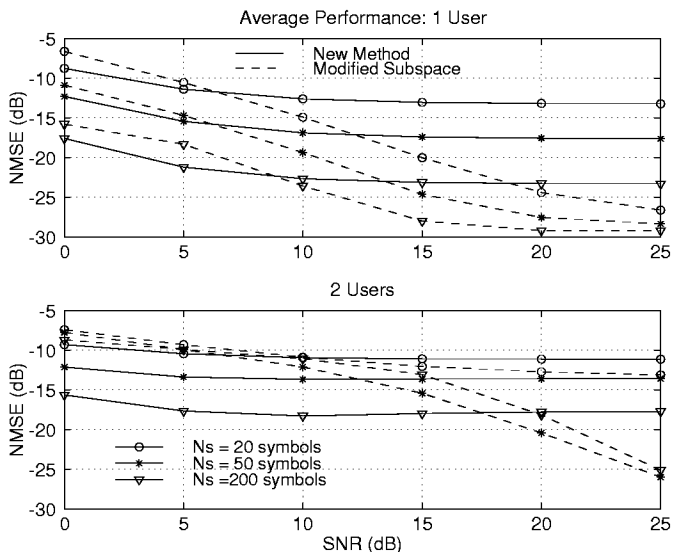
Figure 1. Average performance vs. SNR, 100 randomly generated channels, 100 trials each channel.
