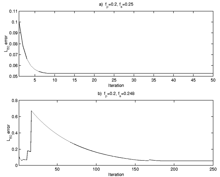
Figure 1: a) BBS method, normal behavior; b) a problematic bandwidth.
