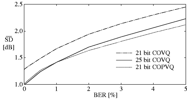
Figure 2: Average SD for 21 bit COPVQ compared with 21 bit and 25 bit memoryless COVQs.
