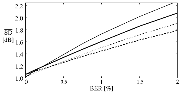
Figure 3: Average SD for 21 bit PVQs with different index assignments. The solid lines correspond to post process IA and the dashed lines to IA obtained by COPVQ design. Two cases are considered: no degradation of noise-free performance allowed (thin lines) and a small degradation of noise-free performance is allowed to improve noisy channel performance (thick lines).
