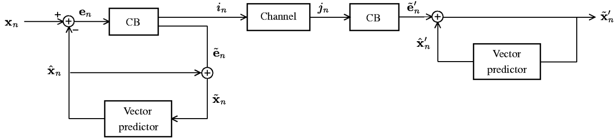
Figure 1: Predictive VQ operating over a noisy channel. A prediction error vector is formed by subtracting from the input vector a prediction of it. The prediction error vector is then quantized by a memoryless VQ.
