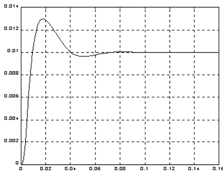
Fig4 Response curve of 0.01^\circ step
