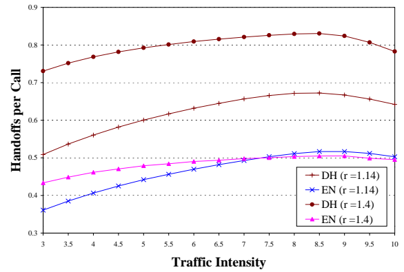
Figure 4: Average number of induced handoffs.
