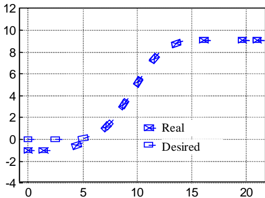
Figure 3: Cartesian motion
