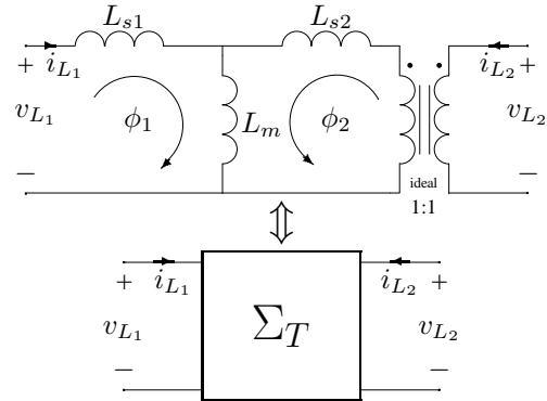
Figure 1: Equivalent topology of a pair of coupled-inductors
