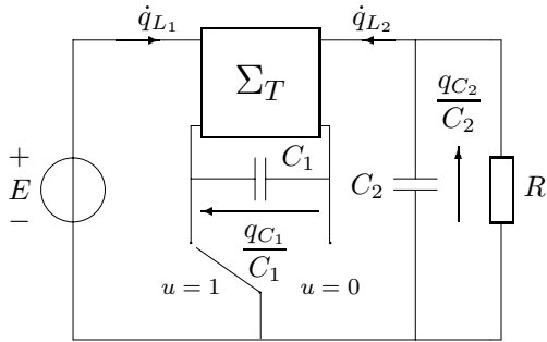
Figure 2: Coupled-inductor Ćuk converter
