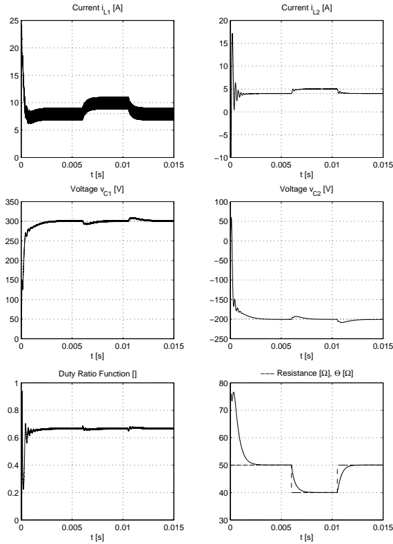
Figure 4: Simulation of the closed-loop passivity-based Ćuk converter with zero-output ripple
