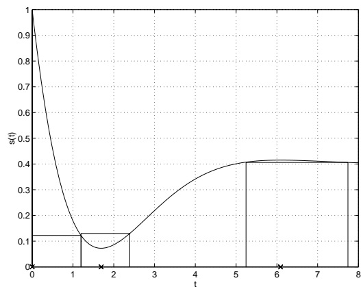
(a) Step response s with calculated position of the pulses for the worst case input.
