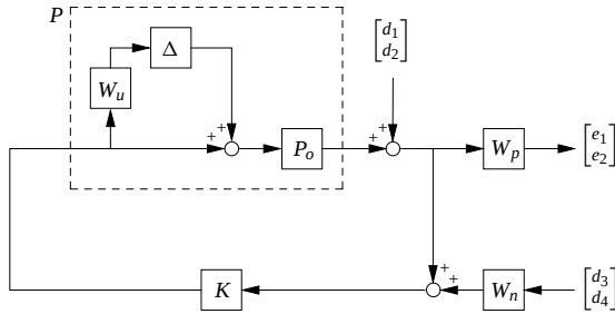
Figure 2: Block diagram of HIMAT and required feedback structure
