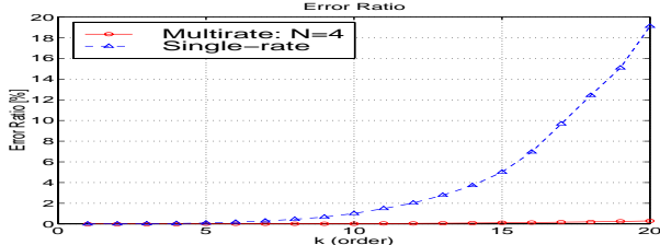
Figure 9: Error ratio E_R(k) . (20th order corresponds to 2.4 [kHz].)
