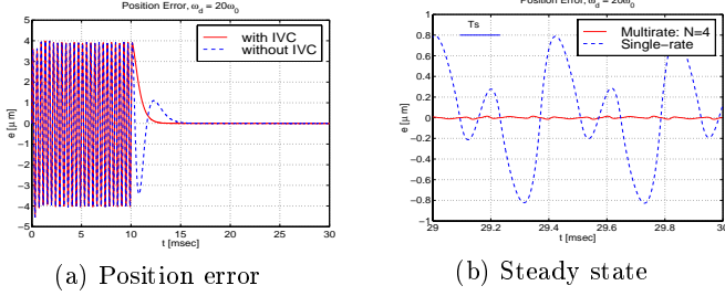
Figure 8: Feedforward repetitive control. d_y(t) = T_p \sin k\omega_0 t , T_p = 3.6\mu\text{m} , k = 20 .
