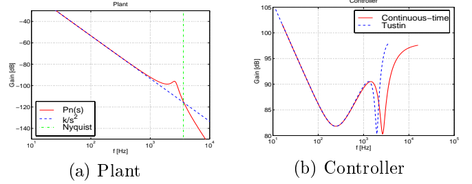
Figure 4: Frequency responses.
