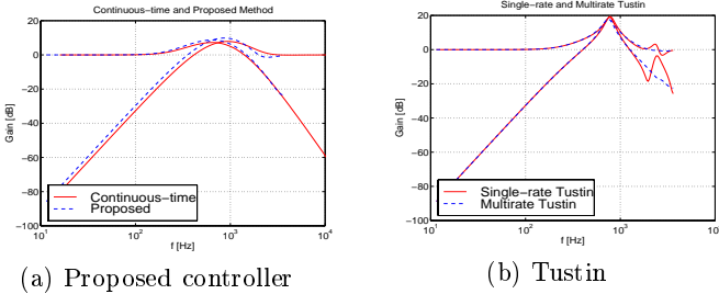
Figure 6: Frequency responses S[z], T[z] .
