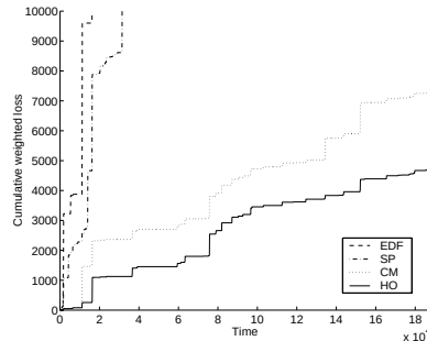
Figure 2: Weighted packet loss for four schedulers
