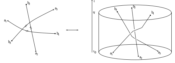
Figure 1: A 3-maneuver and its braid representation.
