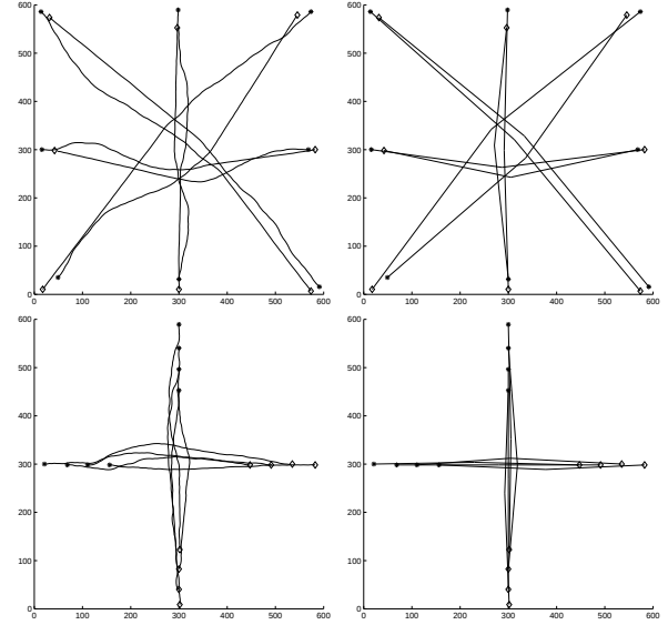
Figure 7: Resolution maneuvers for 8-aircraft encounters.
