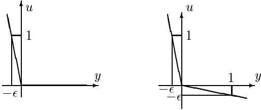
Figure 2: Examples of characteristics that give admissible approximations
