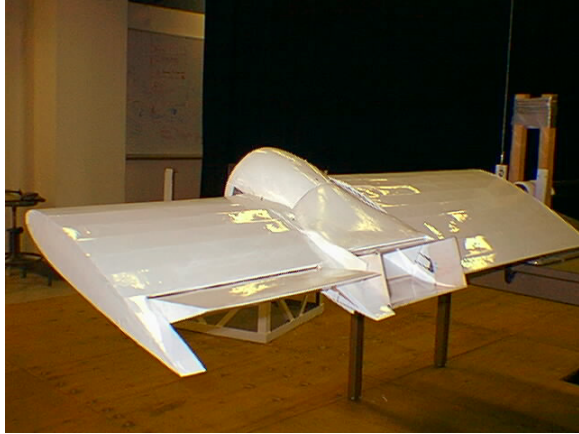
Figure 1: New Caltech Ducted Fan flight vehicle—July 99.
