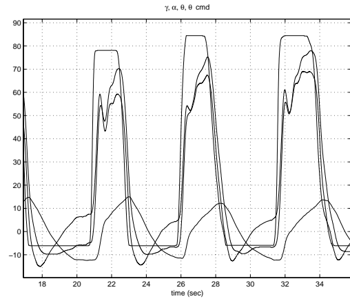
Figure 3: High AOA maneuvering of the Ducted Fan.
