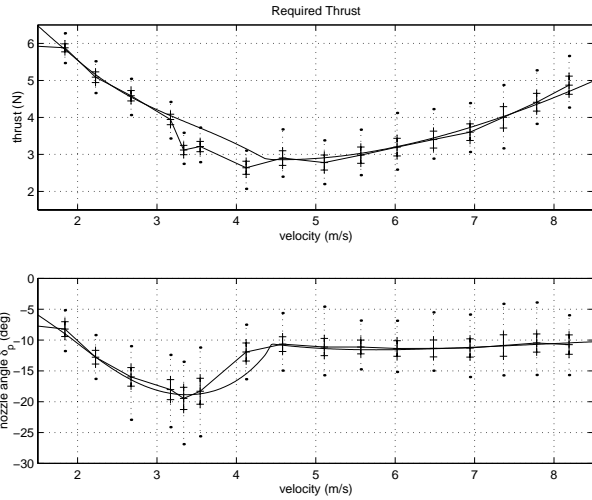
Figure 5: Experimental and model equilibrium manifolds. Required thrust vs. velocity
