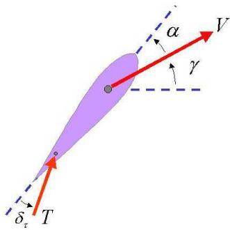
Figure 6: Flying wing with vectored thrust.
