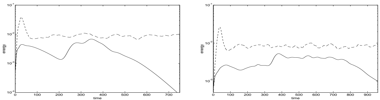
FIG. 4. Control of oblique waves (left) and an initially random flow perturbation (right). The magnitude of the initial flow perturbations in these simulations significantly exceed the thresholds reported by Reddy et al. (1998) that lead to transition to turbulence in an uncontrolled flow (by 225\times for the oblique waves and by 15\times for the random initial perturbation). Solid lines indicate the energy evolution in the controlled case, dashed lines indicate the energy evolution in the uncontrolled case. Both of the uncontrolled simulations result in transition to turbulence whereas both of the controlled systems relaminarize.
