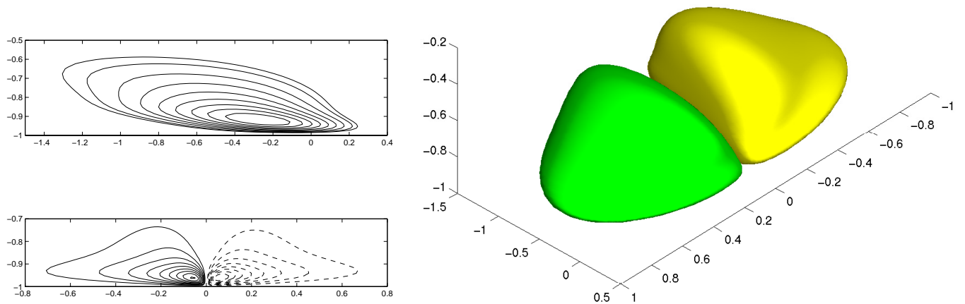
FIG. 3. Physical-space feedback convolution kernel for \omega . Contours of an xy plane at z = -0.3 (top) and a zy plane at x = 0 (bottom) are shown on the left, and two isosurfaces of the convolution kernel are shown on the right.
