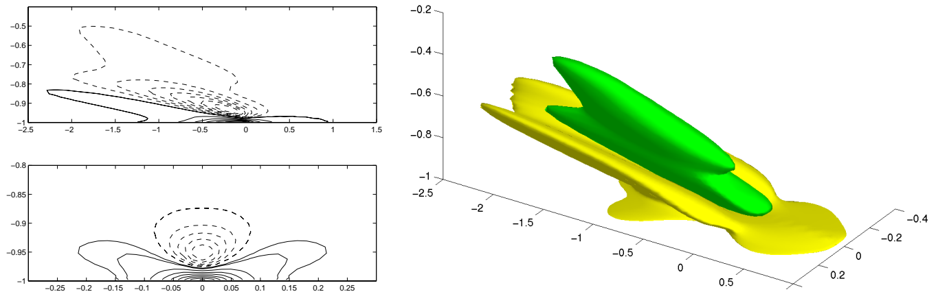
FIG. 2. Physical-space feedback convolution kernel for v . Contours in an xy plane at z = 0 (top) and a zy plane at x = 0 (bottom) are shown on the left (positive contours solid, negative contours dashed), and two isosurfaces of the convolution kernel are shown on the right (one positive and one negative).
