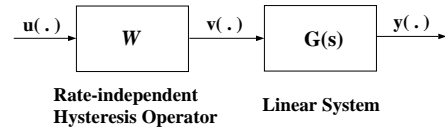
Figure 1: Structure of models for smart actuators
