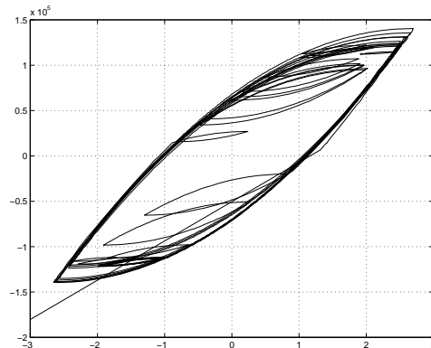
Figure 8: Output versus Input graph shows hysteresis.
