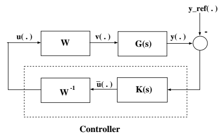
Figure 2: Controller design schematic
