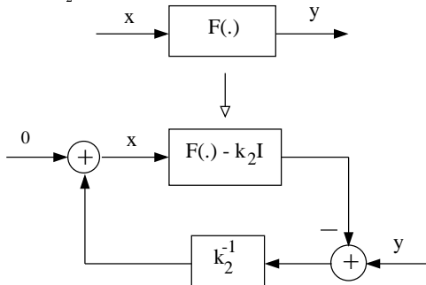
Figure 4: Decomposition of an incrementally strictly increasing system into a feedback system
