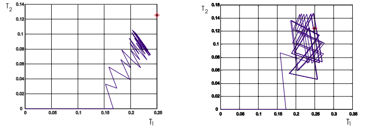
(a) Closed-loop MPC control of system (18) for u_0 = 0.4
