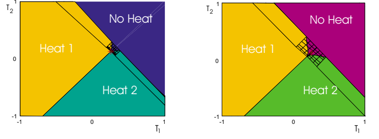
(a) Explicit optimal controller for u_0 = 0.4
