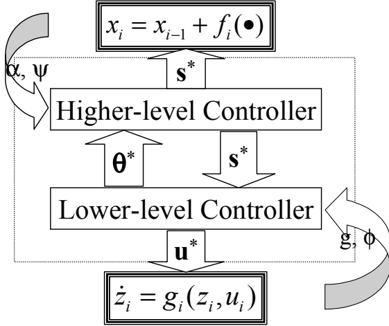
Figure 1: Hybrid Controller Operation
