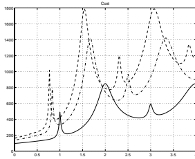
Figure 7 The cost J_i(h) as a function of the sampling interval for a non-inverted pendulum. The plots shows the graphs for \omega_0 = 3.1416 (full), 3.7699 (dot-dashed), and 4.0841 (dashed).
