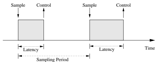
Figure 1 Basic timing constraints of a control loop.
