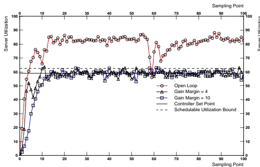
Figure 3: Utilization Control Performance
