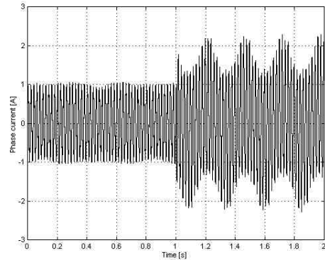
Fig. 4 Current signal for normal unloaded behaviour followed by loaded faulty behaviour
