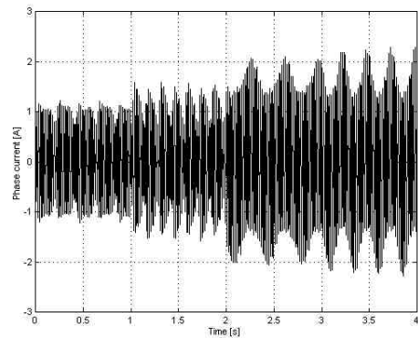
Fig. 5 Current signal for increasing load abnormal behavior.
