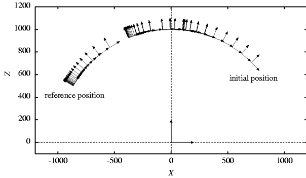
Fig. 6. Camera position
