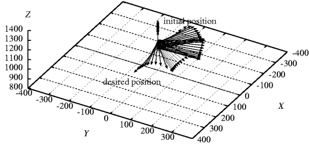
Fig. 10. Camera position
