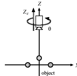
Fig. 3. Camera motion (2D rotation)
