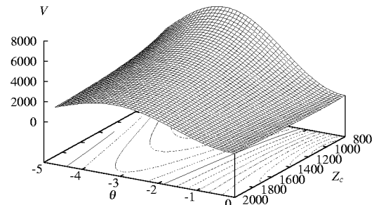
Fig. 4. Potential plot (2D rotation)
