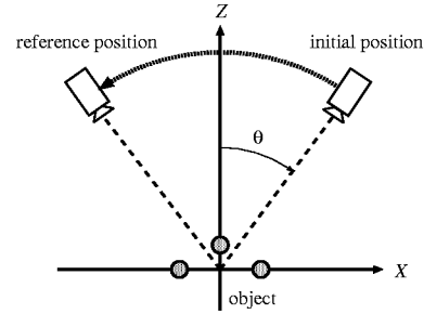
Fig. 1. Camera motion (circular)
