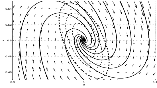
Figure 2: Example 2: a = 0.5 , b = 0.5 . Solid lines show trajectories, dotted curves are level curves of the Lyapunov function
