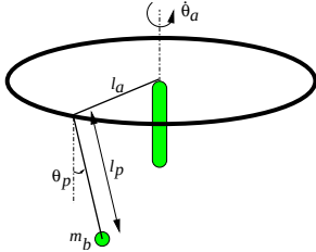
Figure 4: The whirling pendulum
