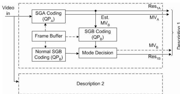
Fig. 2 Structure of proposed SG-MDC
