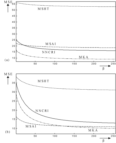
Fig. 2. Performance (MSE) of the proposed normalized color-ratio based interpolators depending on \beta : (a) the test image Lighthouse, (b) the test image Butterfly.
