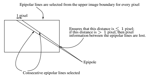
Fig. 6. Loss of pixel information occurs when the maximum distance between two consecutive epipolar lines are > 1 pixel. In our method, by choosing the correct image boundaries to scan, this is prevented.
