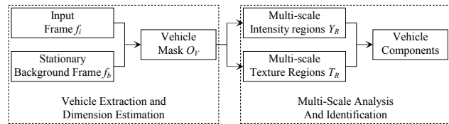
Fig. 1: Scale space identification of vehicle components
