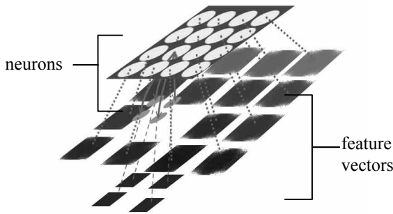
Fig. 2. The architecture of our SOM network. Solid lines indicate the links between parent-nodes and child-nodes while dotted lines map neurons to feature vectors expressed in images.
