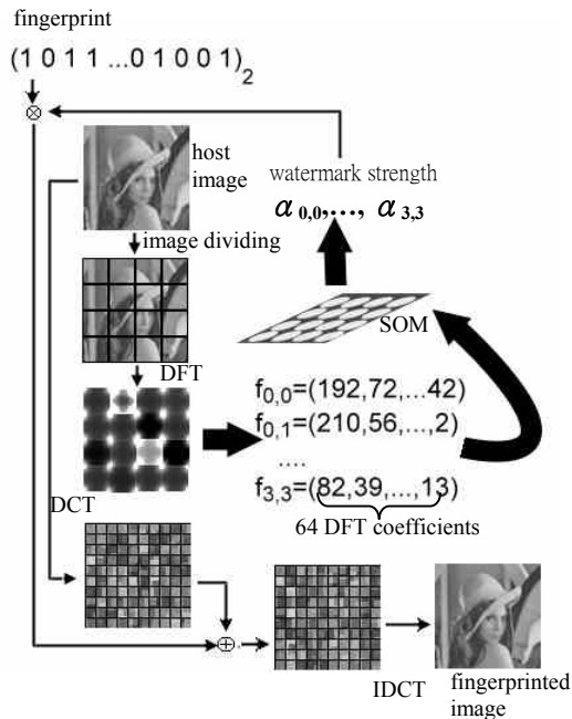
Fig. 3. The fingerprint embedding process.
