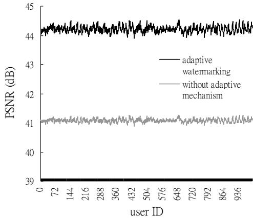
Fig. 4. Imperceptibility comparisons between the adaptive watermarking and the naïve watermarking schemes with fixed strength.
