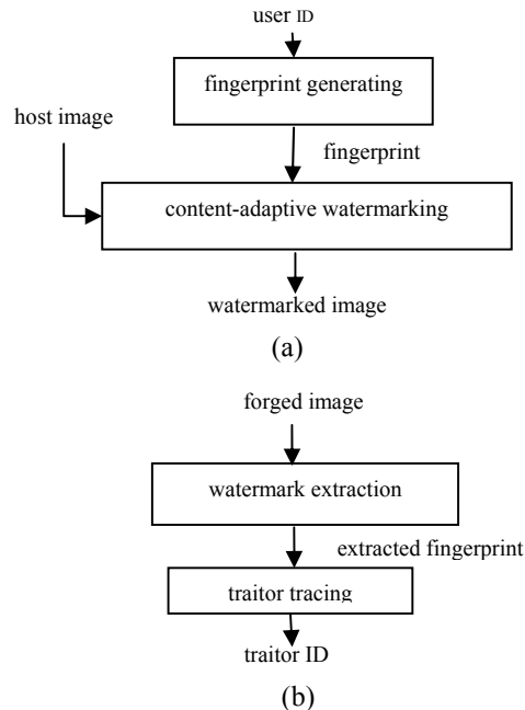
Fig. 1. System overview. (a) fingerprinting scheme. (b) traitor tracing scheme.
