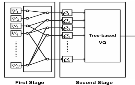
Fig. 1. The proposed two-stage-VQ structure.
