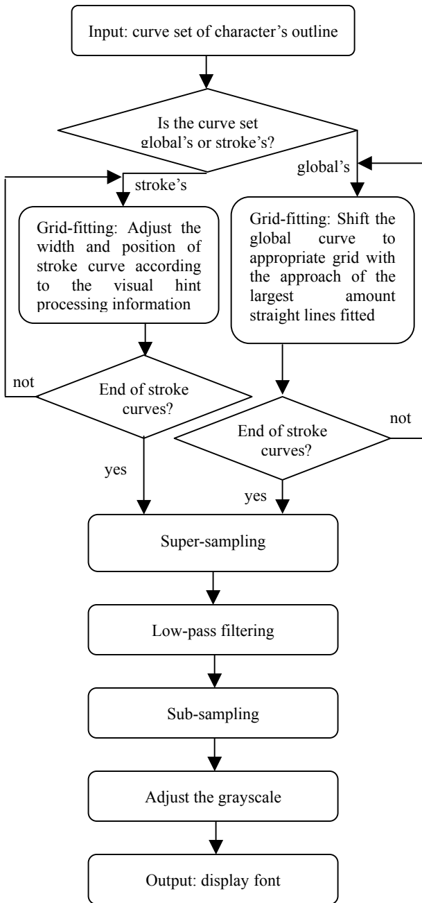
Figure 1. The proposed display algorithm for small-size Chinese characters.
