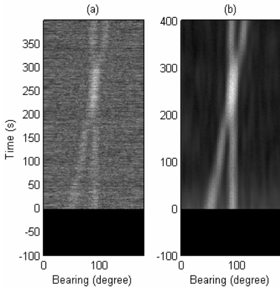
Figure 5: (a) Bearing time record by a real-time sonar system; (b) the proposed method is integrated in the sonar system.
