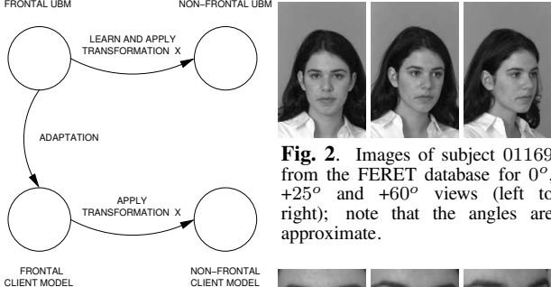
Fig. 1. Graphical interpretation of synthesizing a non-frontal client model based on how the frontal UBM is transformed to a non-frontal UBM.
