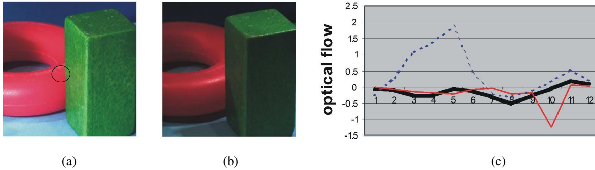
Figure 2: a) frame 1 with filters superimposed on it b) frame 10 c) estimated optical flow over time on the x-position which is indicated in a), with RGB (dotted line), shadow-shading invariant (red line), and shadow-shading and specularity invariant (thick black line).
