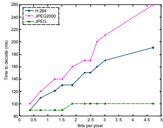
Fig. 4 Time to decode
