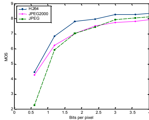
Fig. 2 Subjective Quality
