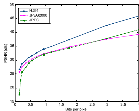
Fig. 1 Objective Quality
