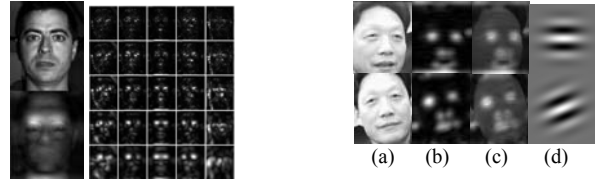
Fig. 4. The eye-and-brow selectivity of some Gabor kernel. Top-left: the original face image. Top-right: the magnitude domain after the Gabor transform. Bottom-left: the original image mixed with the magnitude domain transformed by the horizontal-orientation and fifth-scale kernel
