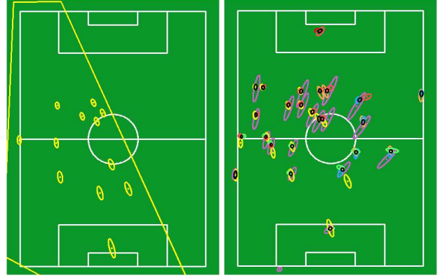
Fig. 3. Measurement covariance (left) from a single camera and (right) from multiple cameras with data integration (black ellipses).
