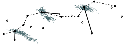
Fig. 5. Three example particle-based posterior distributions for the same realization as Fig. 4, at time t = 2, 5, 8 .
