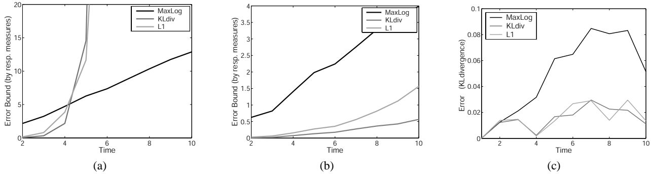
Fig. 6. (a) Error bounds at each time step resulting from a KD-tree based optimization for ML, KL, and L_1 error subject to a maximum of 5 final mixture components. (b) Error bounds for M = 10 mixture components. Notice the change in scale from (a)—improving the quality of each approximation increases the time scale on which the KL and L_1 -based bounds are useful. (c) Increase in actual error (measured by the KL-divergence) due to density approximation for M = 5 .
