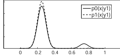
Fig. 3. Given two distributions p^0(x_1|y_1) and p^1(x_1|y_1) with relatively small L_1 error, a new observation y_2 can either increase (if y_2 = 1 ) or decrease (if y_2 = 0 ) the L_1 error between p^0(x_1|y_1, y_2) and p^1(x_1|y_1, y_2) , though one can bound the error in expectation over y_2 ; see text for details.
