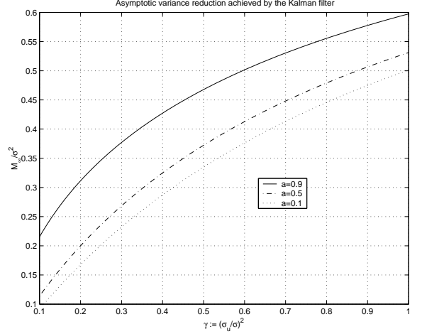
Fig. 3. Variance reduction achieved by a KF versus \gamma := \sigma_u^2/\sigma^2 . The smaller \sigma_u^2 is relative to \sigma^2 , the more effective KFs are.
