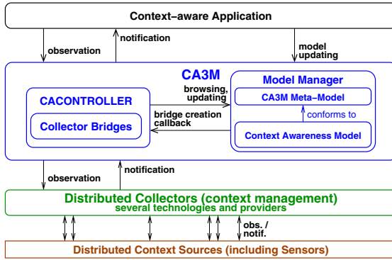
Fig. 2. Runtime architecture of CA3M
