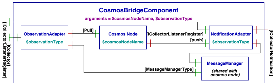
Fig. 7. The COSMOS Bridge component
