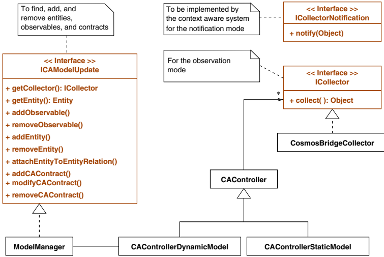
Fig. 6. CA3M related application interfaces
