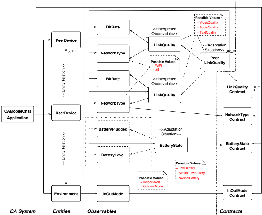
Fig. 4. The context-awareness model for the mobile-chat application
